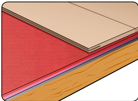
Flooring Devidry™ Wooden floor construction
